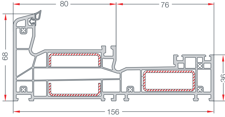
MASTERLINE YALITIMLI SÜRME KANAT PROFİLİ MASTERLINE INSULATED SLIDING FRAME PROFILE EN 342
