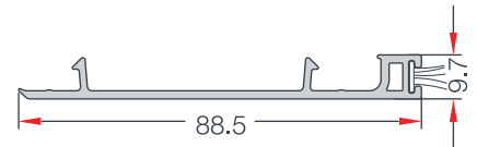
KANAT ARKA KAPAK PROFİLİ SASH COVER PROFILE AKS 1146
